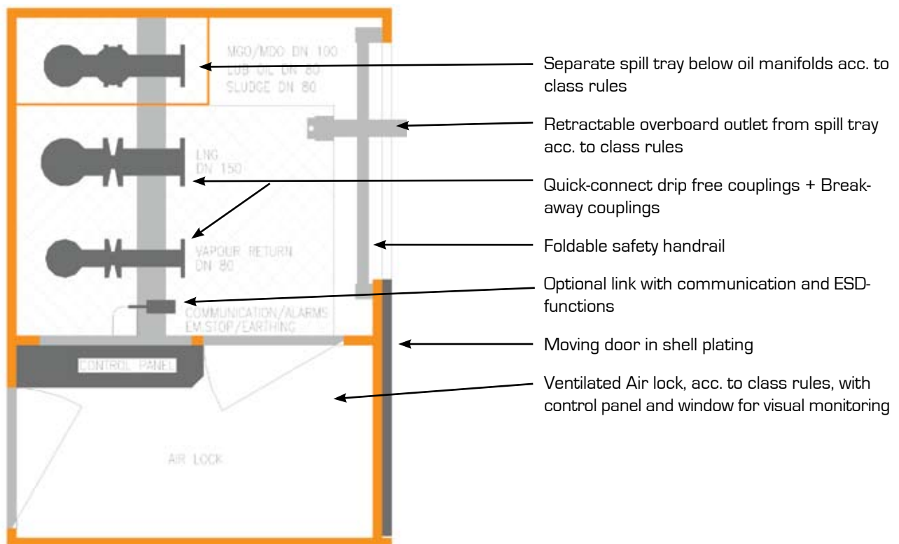
Fig.6 - Recommended Layout of Bunker Station (Receiving ship)
